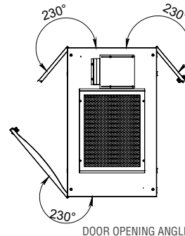
DOOR OPENING ANGLE
