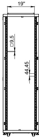
FRONT VIEW WITHOUT DOOR
