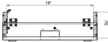
Front View Without Door
